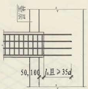
桩顶纵筋在承台内的锚固构造
