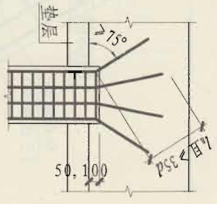
桩顶纵筋在承台内的锚固构造
